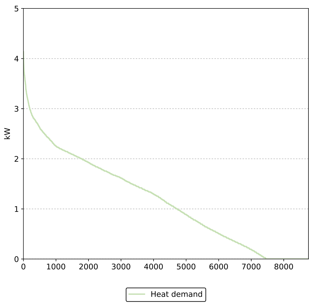
Figure 23: Duration curve of the space heating demand for a building
